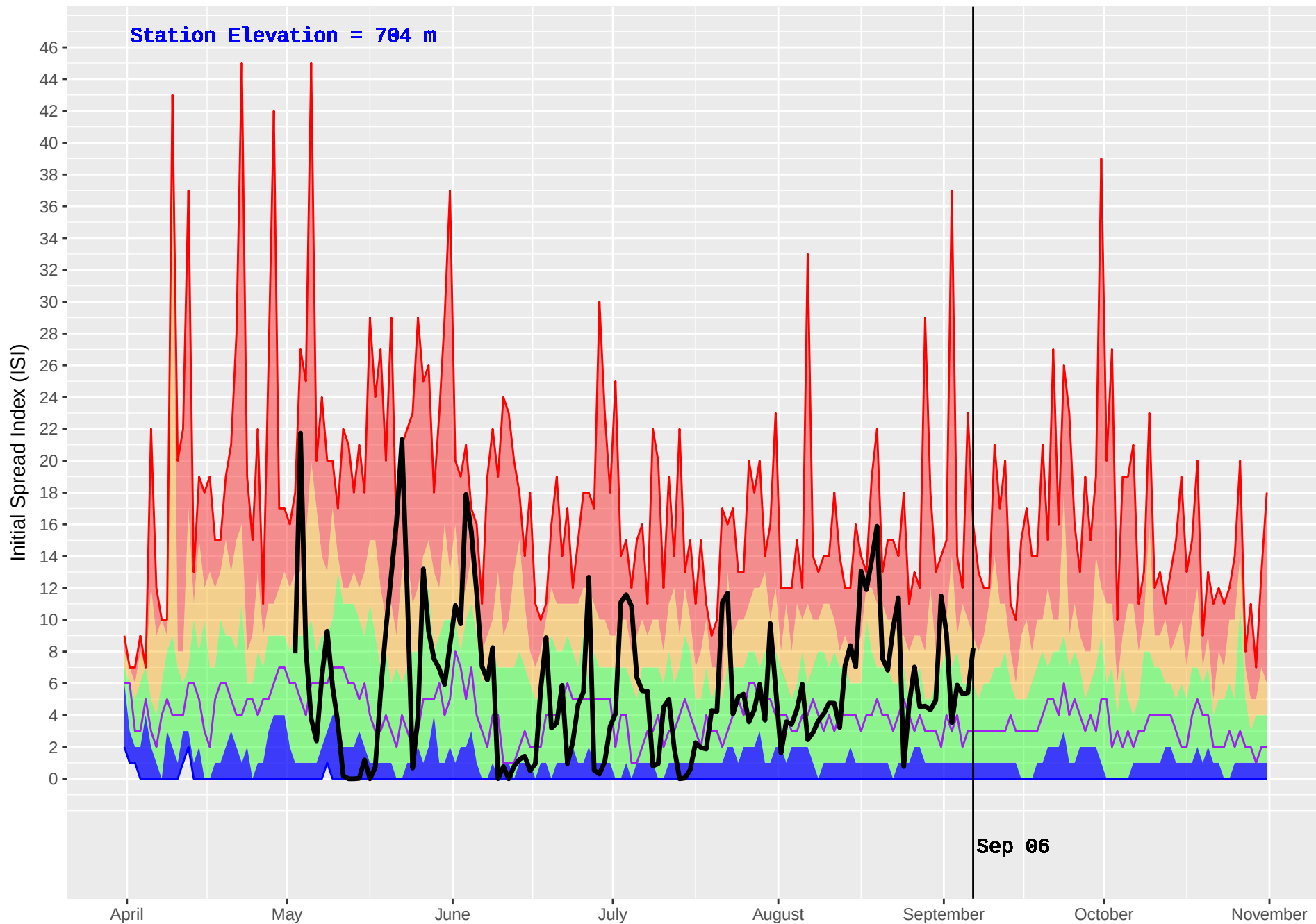
HUDSON HOPE (132) : Historical (1986–2016) and Current (2017) Noon Initial Spread Index (ISI)
