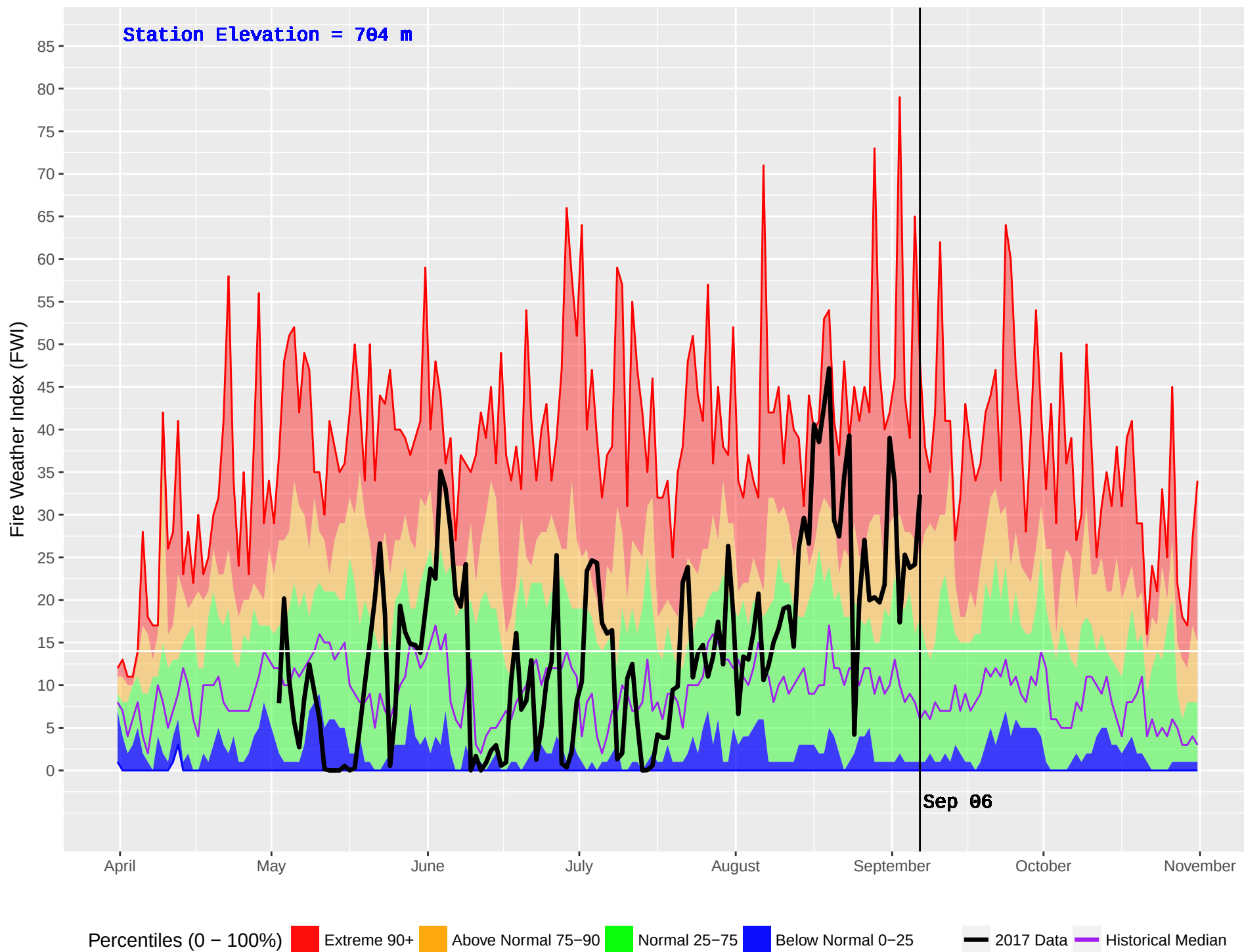
HUDSON HOPE (132) : Historical (1986–2016) and Current (2017) Noon Fire Weather Index (FWI)
