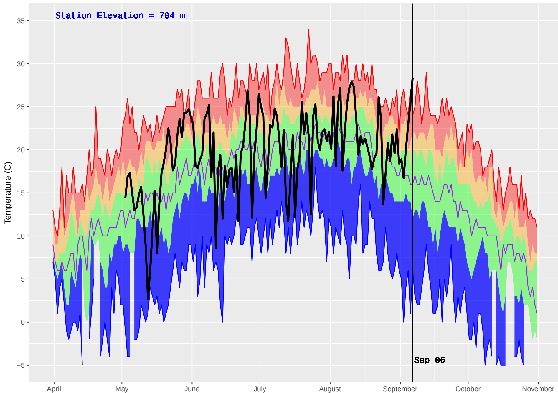
HUDSON HOPE (132) : Historical (1986–2016) and Current (2017) Noon Temperature
