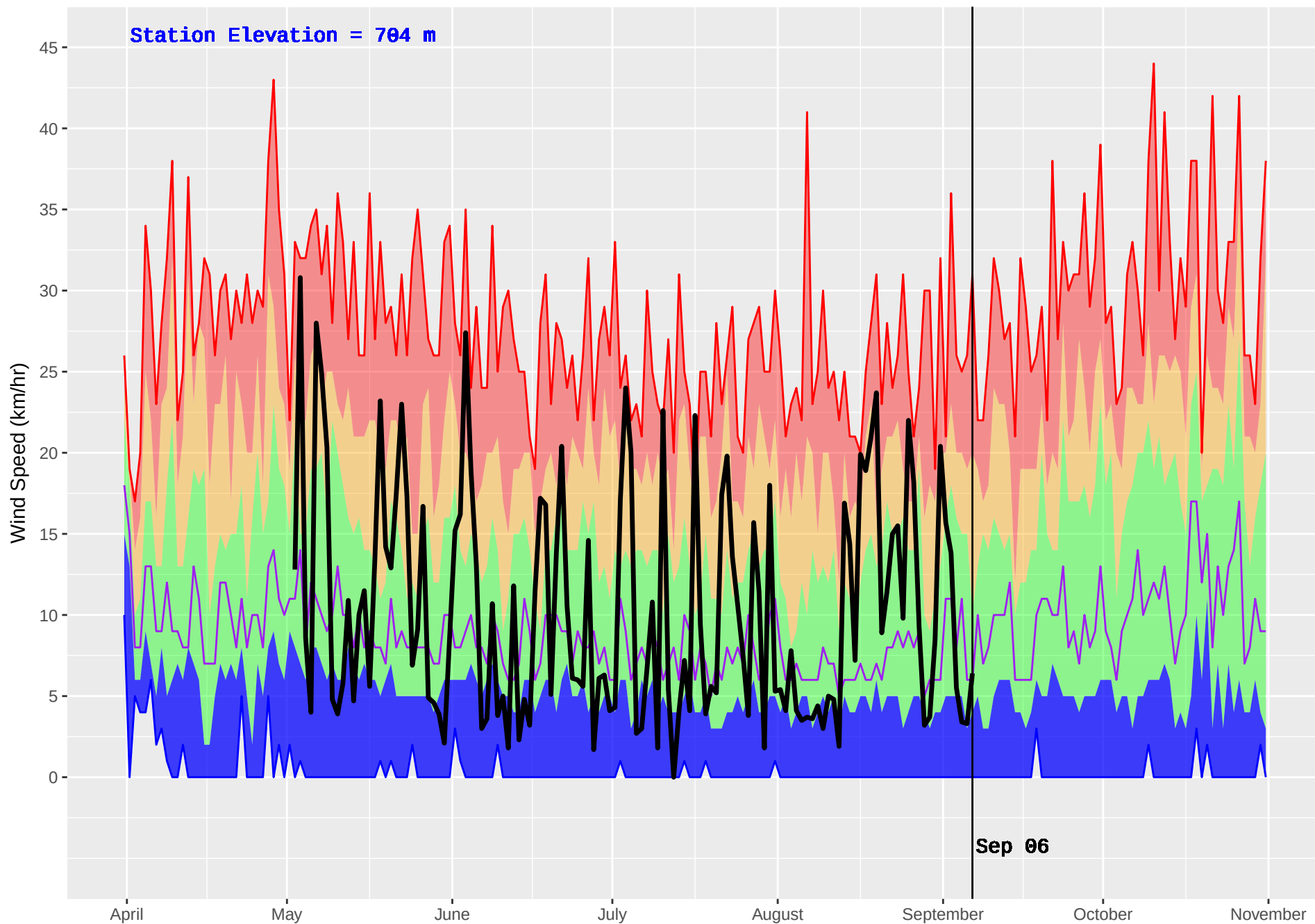
HUDSON HOPE (132) : Historical (1986–2016) and Current (2017) Noon Wind Speed
