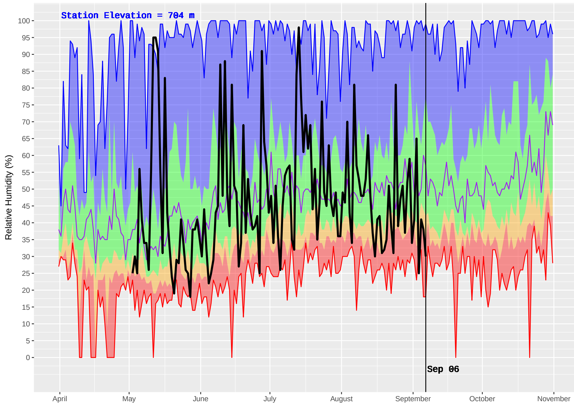
HUDSON HOPE (132) : Historical (1986–2016) and Current (2017) Noon Relative Humidity
